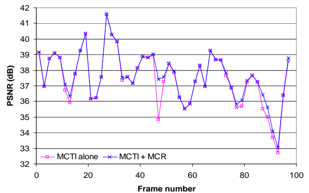
Figure 6. PSNR of every WZ frame in the simulation of the Foreman sequence 30Hz QCIF, with and without MCR.
