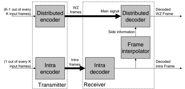
Figure 1. General scheme for a non-iterative DVC codec.
