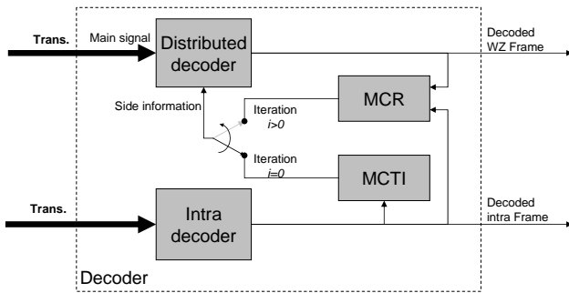
Figure 3. General scheme for the DVC decoder, using iterative side-information generation.
