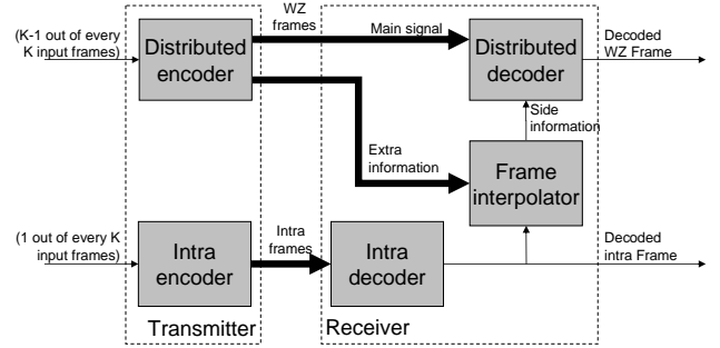
Figure 2. General scheme for a DVC codec using motion-compensated interpolation with extra information.
